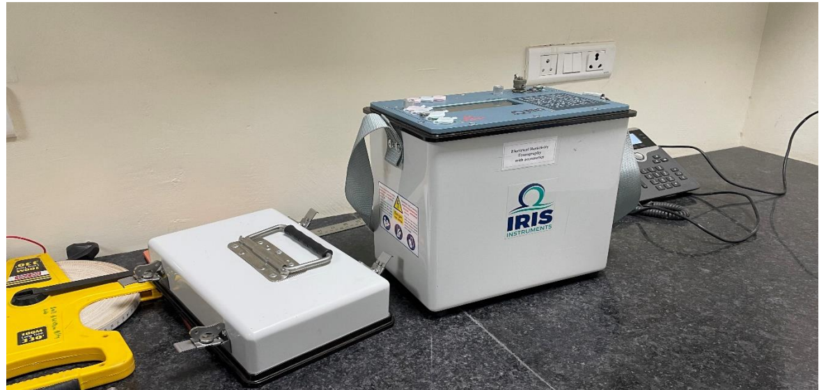
Electrical Resistivity Tomography Equipment
